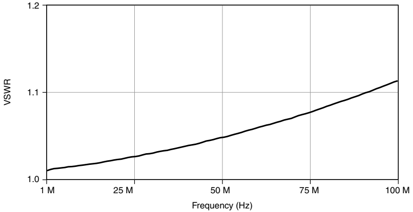
Figure 2. 50 \Omega Input Return Loss, Characteristic
