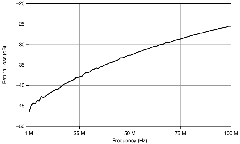
Figure 2. 50 \Omega Input Return Loss, Characteristic
