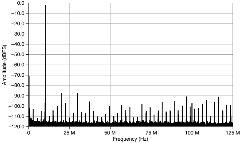
Figure 4. 50 \Omega Single-Tone Spectrum, 1.4 V pk-pk Input Range, Full Bandwidth, 9.9 MHz Input Tone at -1 dBFS, Characteristic
